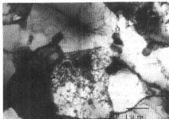
Fig.5 Microstructure of HE sample at 873 K for 350 h
