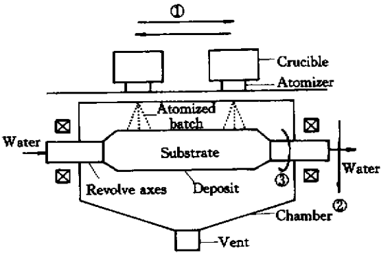
Fig. 1 Schematic of multi-layer spray deposition device
