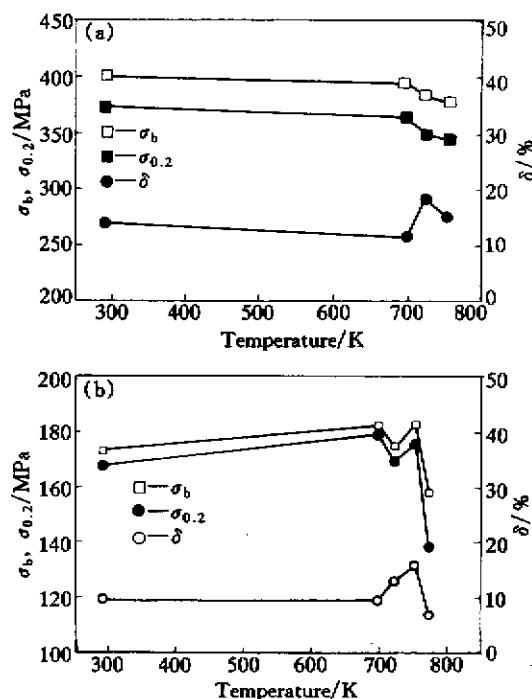
Fig. 3 Mechanical properties of HE alloy at different temperatures for 500 h
