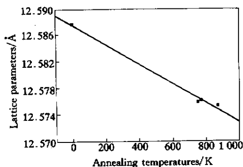
Fig. 6 Lattice parameters of \text{Al}_{12}(\text{Fe}, \text{V})_3\text{Si} phase after HE for 500 h vs annealing temperature
