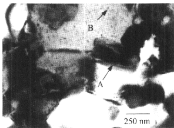
Fig.4 Typical microstructure of warm extruded sample
